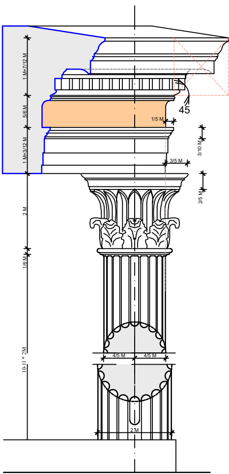
GREEK CORINTHIAN ORDER TOWER OF THE WINDS
