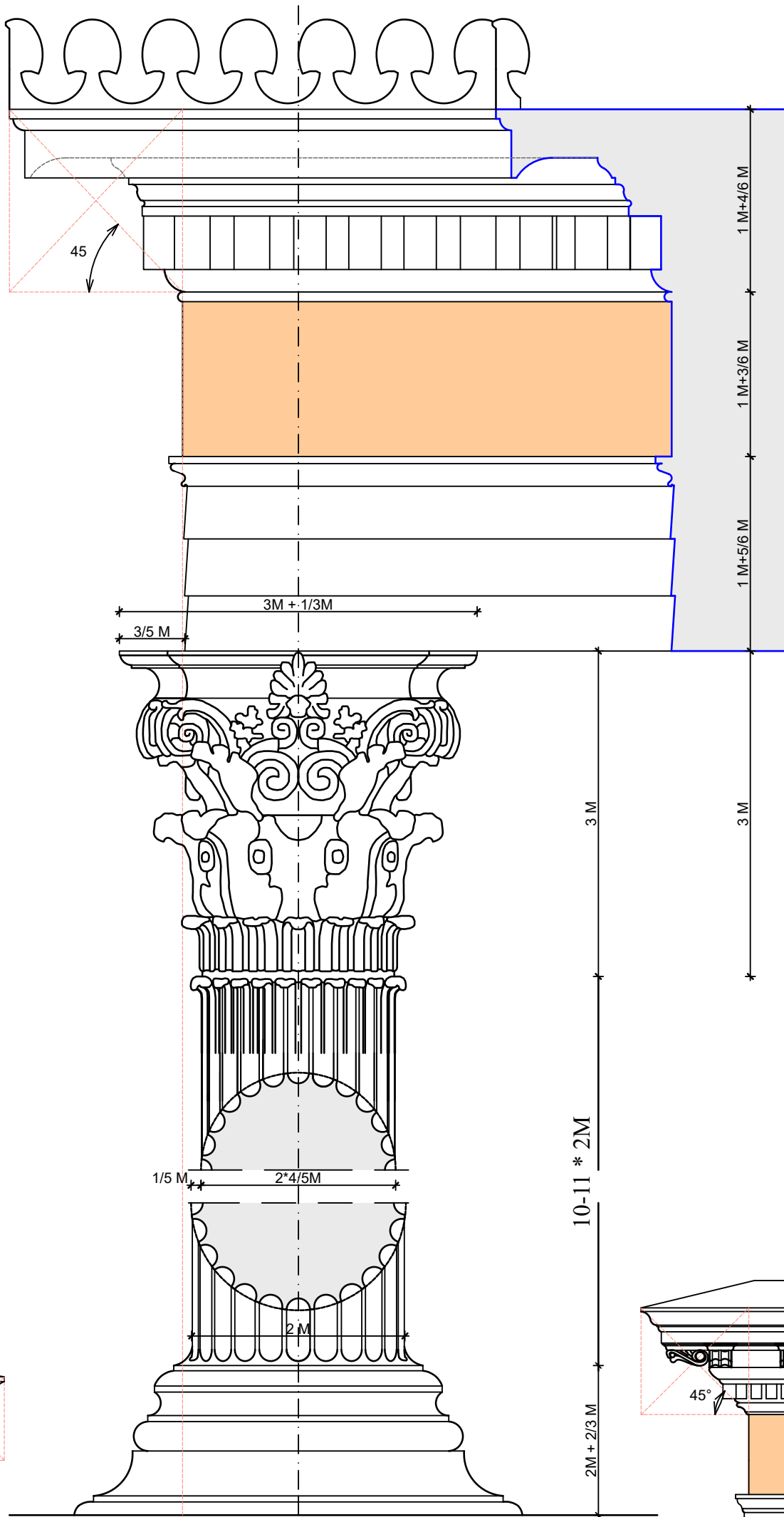
GREEK CORINTHIAN ORDER LYSICRATES MEMORIAL
