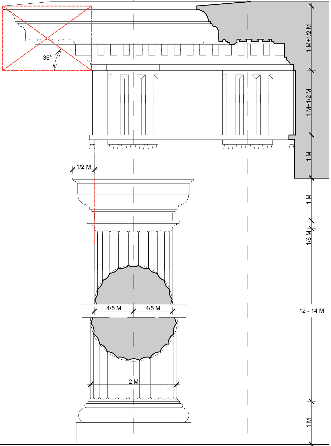
ROMAN DORIC ORDER
